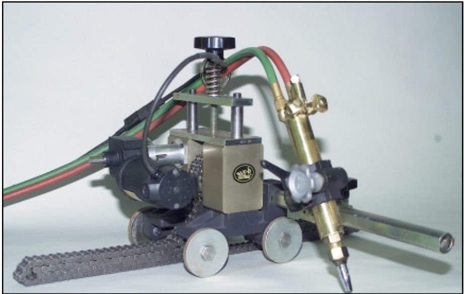
Motorized Pipe-Bug 110V. Part # BUG-05-0520-M00 Weight: 42lbs (19kg) Shipping Weight: 47 lbs. (22kg) Motorized Pipe-Bug 230V. Part # BUG-05-0520-ME2 Weight: 56 lbs. (26kg) Shipping Weight: 61 lbs. (28kg)
