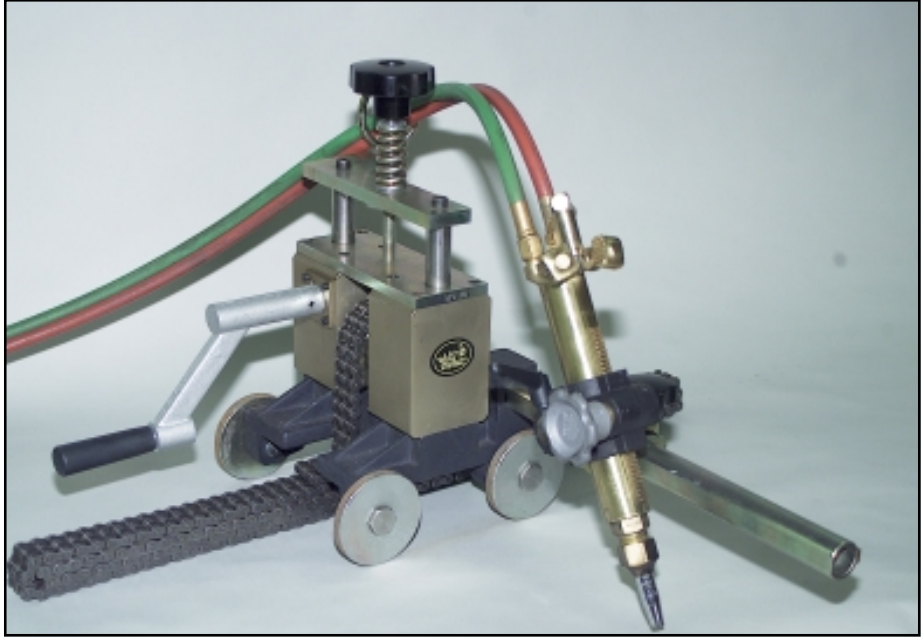
Manual Pipe-Bug. Part # 05-0520-000 Weight: 34 lbs. (16kg) Shipping Weight: 39 lbs. (18kg)
